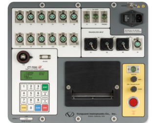
CT-7000 S2 Digital Circuit Breaker Analyzer
