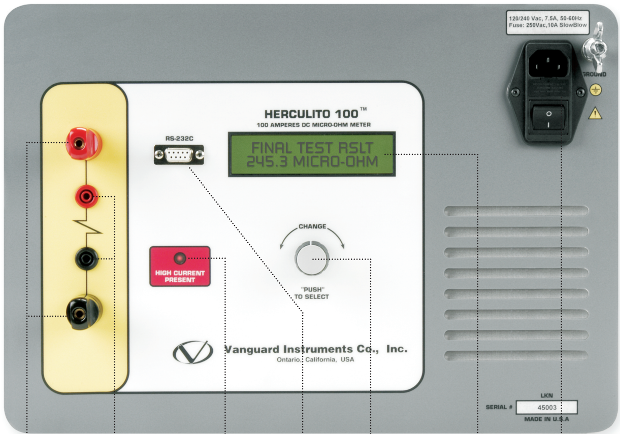
Current Lead Connector Sensing Lead Connector High Current Presence Indicator RS-232C Interface Function Control Knob Back-lit LCD Screen (16 characters by 2 lines) Built-in Circuit Breaker
